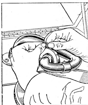
Insert Needle
